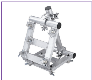
BOOK CORNER-12 Variable Degree Angle Corner AVAILABLE IN BLACK & WHITE POWDER COAT
