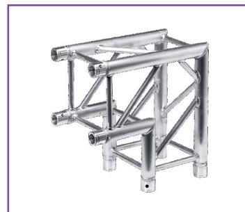
SQ-4I21 1.64ft (0.5m) 2 90° Corner AVAILABLE IN BLACK POWDER COAT
