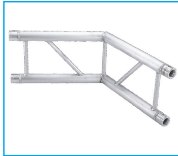
IB-4061V 1.64ft (0.5m) 2 Way 120° Vertical Corner
