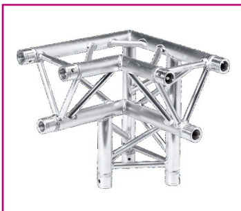
TR-4093/DR 1.64ft (0.5m) 3 Way 90° Triangular Corner Apex down/right
