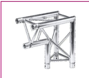
TR-4088/I 1.64ft (0.5m) 2 Way 90° Triangular Corner Apex in
