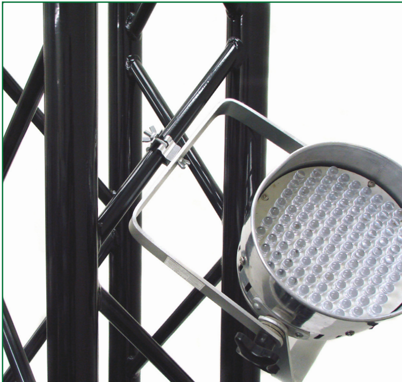
MINI-360-FI4 USED ON F34 TRUSS DIAGONAL BRACE
