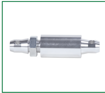
SPACER 5019 105 - 170 mm / 4.1 - 6.7 in
