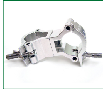
JR SWIVEL CLAMP Unit Weight: 1 lbs. Max Weight Capacity: 75 kg. / 165 lbs. TUV Approved
