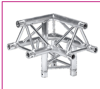
TR-4093/UR 1.64ft (0.5m) 3 Way 90° Triangular Corner Apex up right
