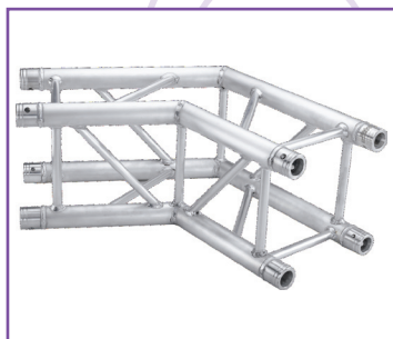
SQ-4I22 1.64ft (0.5m) 2 Way 120° Corner
