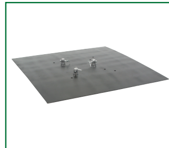
BASEPLATE 3.3S 3 ft X 3 ft Steel Baseplate 95 lbs Will ONLY work with F33/F34/F44P
