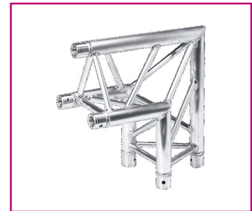
TR-4088/O 1.64ft (0.5m) 2 Way 90° Triangular Corner Apex out
