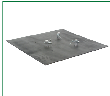
BASEPLATE 2.2S 2 ft x 2 ft Steel Baseplate 50 lbs Will ONLY work with F24/F33/F34
