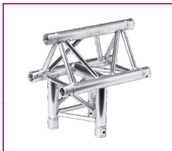
TR-4096H-O 1.64ft (0.5m) 3 Way Triangular Horizontal T-Junction Apex out
