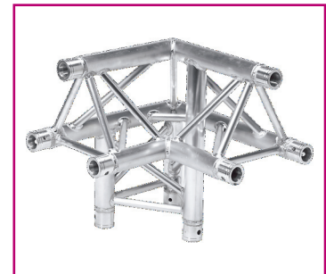
TR-4093/UL 1.64ft (0.5m) 3 Way 90° Triangular Corner Apex up left
